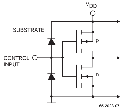
Figure 5. Equivalent Input Circuit
