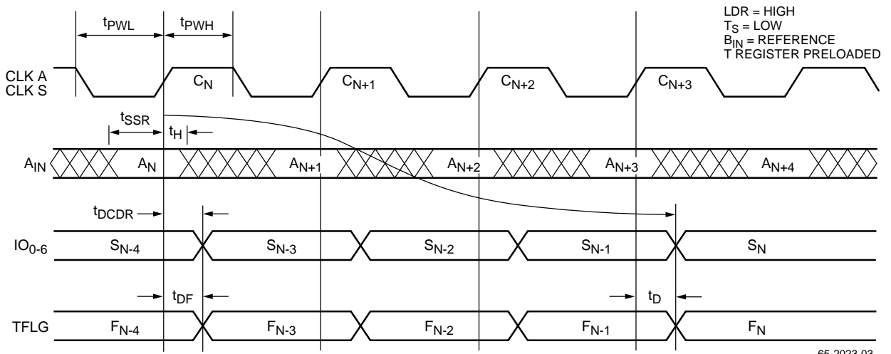
Figure 1. Continuous Correlation
