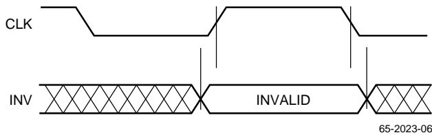
Figure 4. Invert Control Timing
