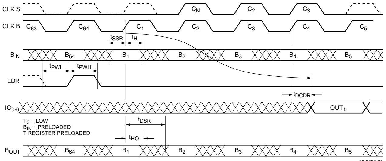
Figure 2. Cross-Correlation
